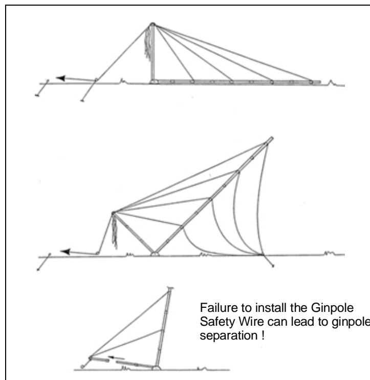
Figure 7: Tower Tilt-up Sequence
