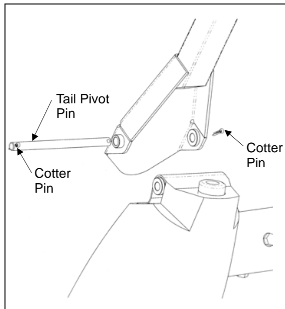
Figure 14: Tail Boom Attachment
