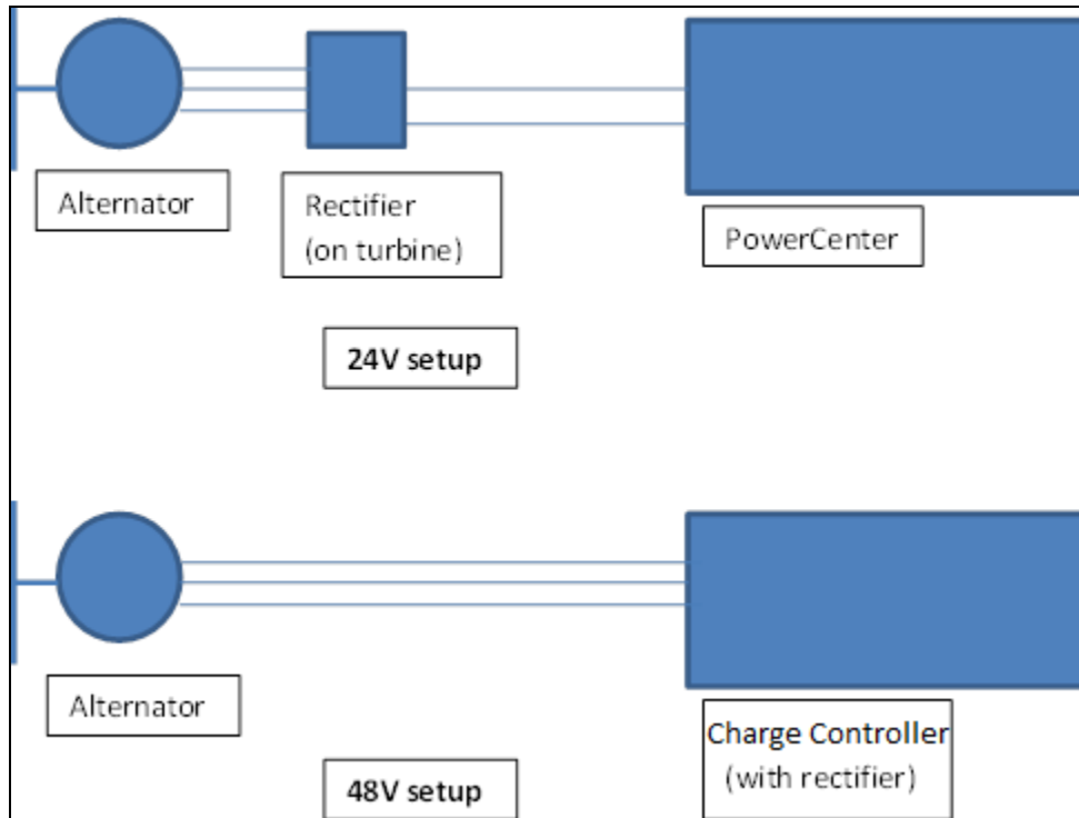
Figure 9: EXCEL 1 Wiring Schematics
